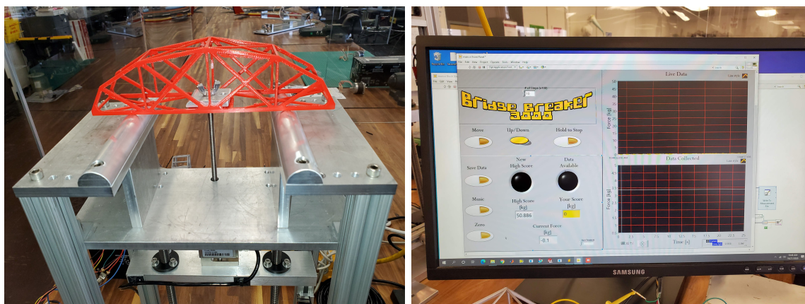
Figure 28. Photos of bridge testing apparatus (left) and testing display (right). A slow-motion video of a test run is available at https://photos.app.goo.gl/MYNW1awqcMDmwHYx8 .
