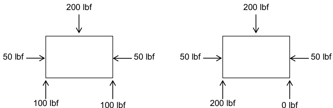
Figure 3. Two sets of forces on an object, both satisfying \Sigma F_x = 0 and \Sigma F_y = 0 , but one (left) in static equilibrium, the other (right) not in static equilibrium.
